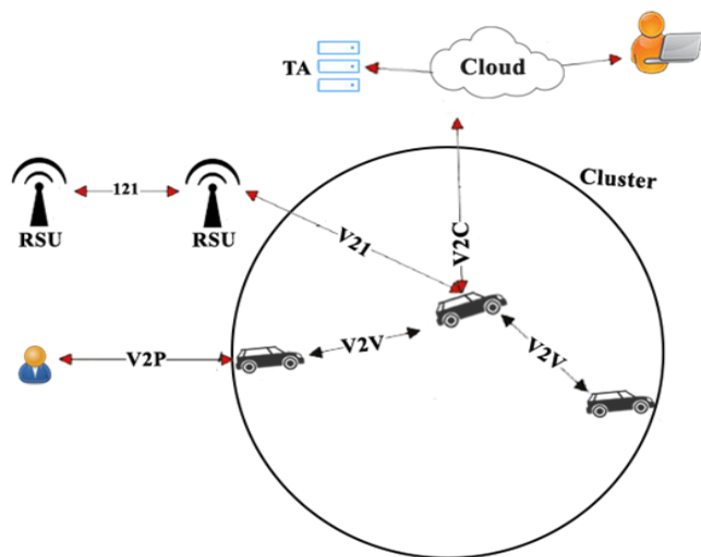
Fig.2. Iov Communication [6]
